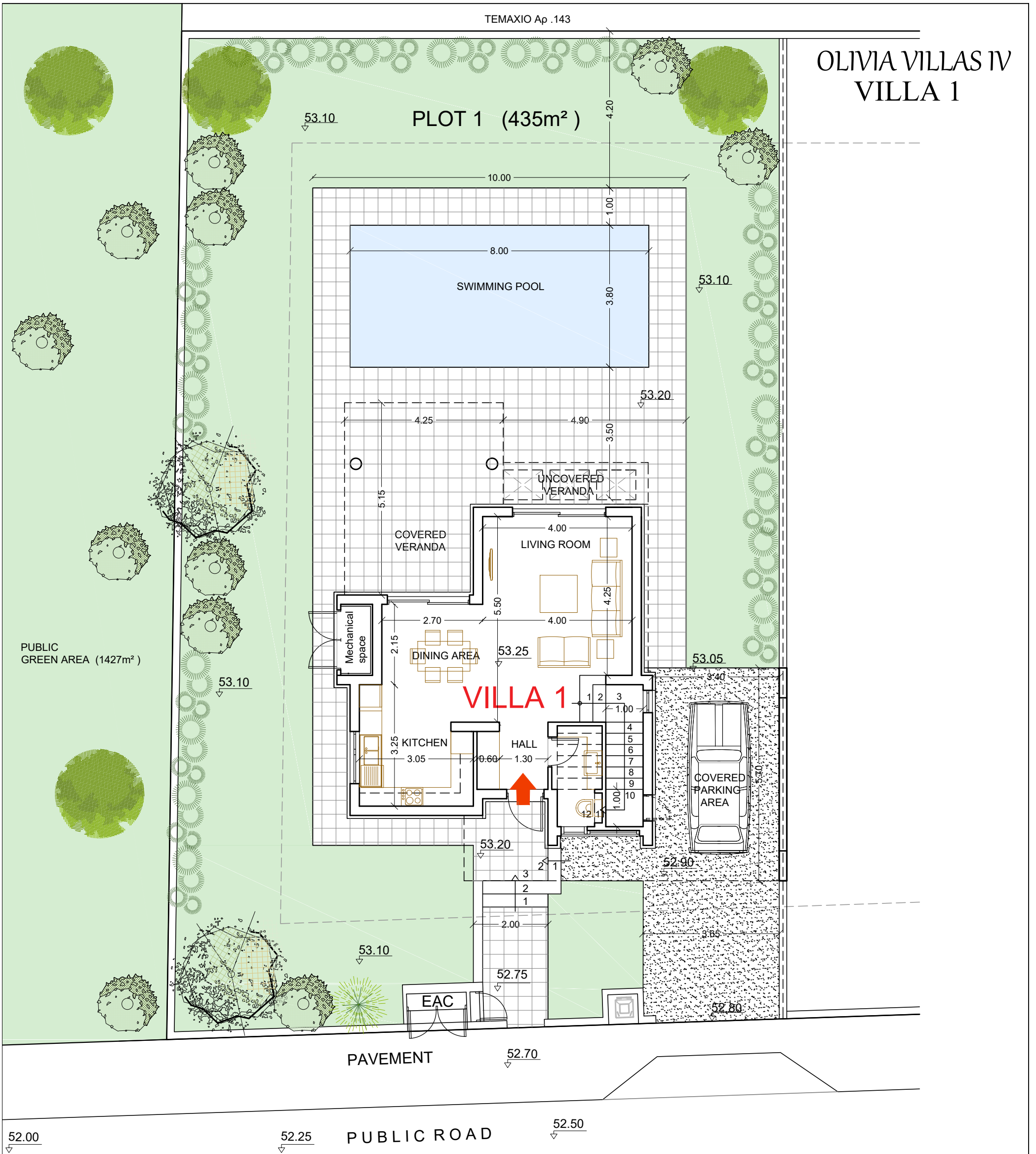
GROUND FLOOR PLAN SITE PLAN
